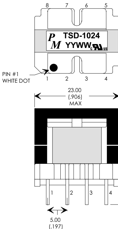
FIGURE 2: PHYSICAL DIMENSIONS mm (INCHES)
