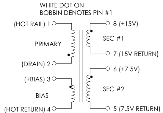
FIGURE 1: SCHEMATIC DIAGRAM
